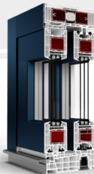
CAPOTAGE ALUMINIUM
